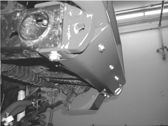
Photo Shown With Optional Steering Box Skid Plate
